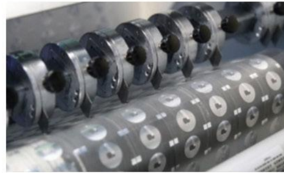
Die-Cutting
