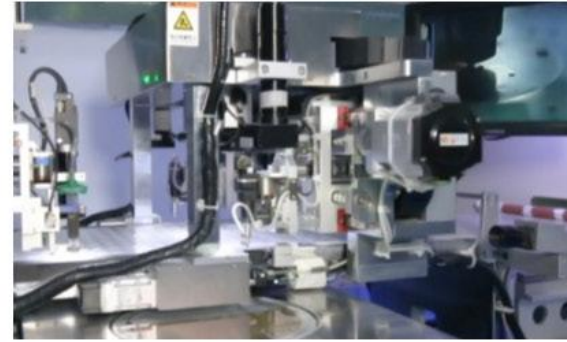
Flip-Chip
